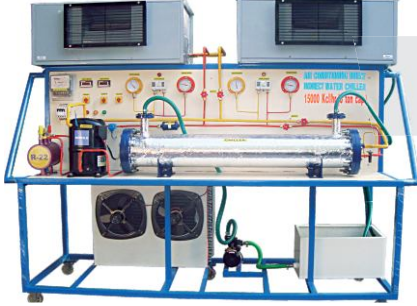
Air Conditioner Direct / Indirect Chiller Capacity : 5 ton
